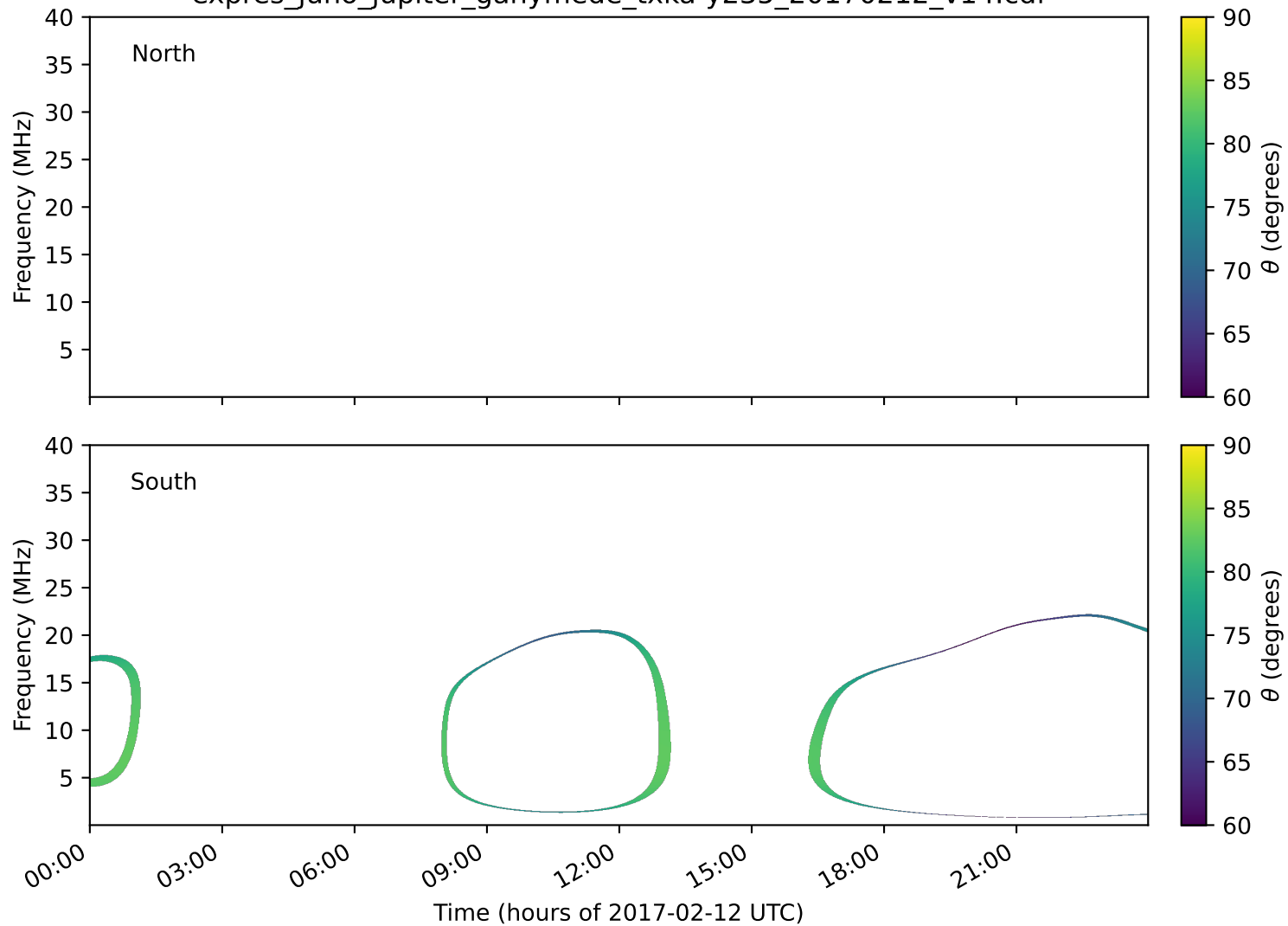
expres_juno_jupiter_ganymede_txka-y235_20170212_v14.cdf
