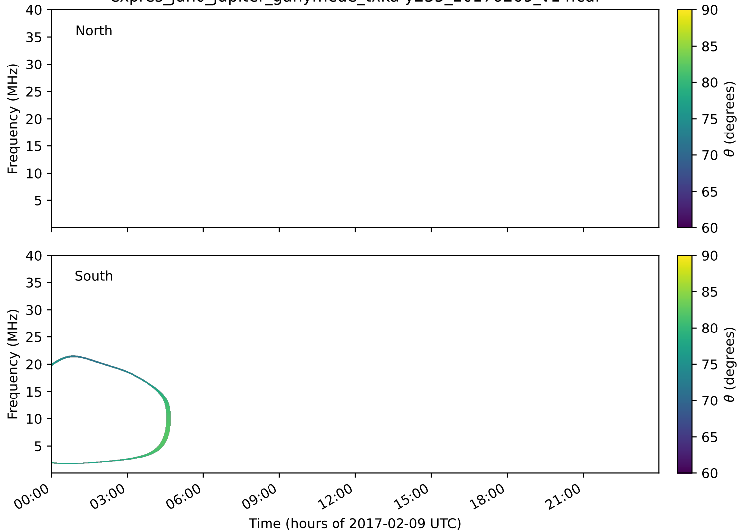
expres_juno_jupiter_ganymede_txka-y235_20170209_v14.cdf
