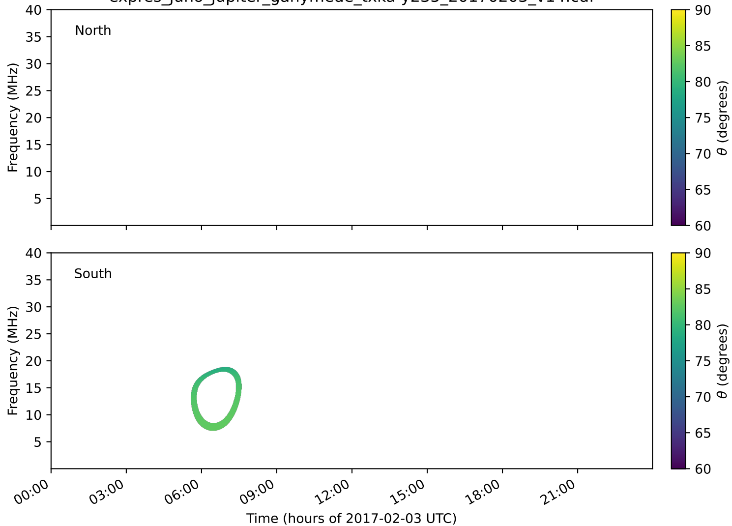
expres_juno_jupiter_ganymede_txka-y235_20170203_v14.cdf
