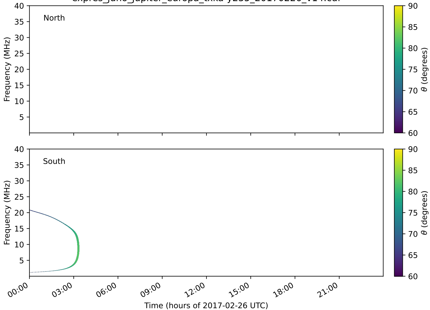
expres_juno_jupiter_europa_txka-y235_20170226_v14.cdf
