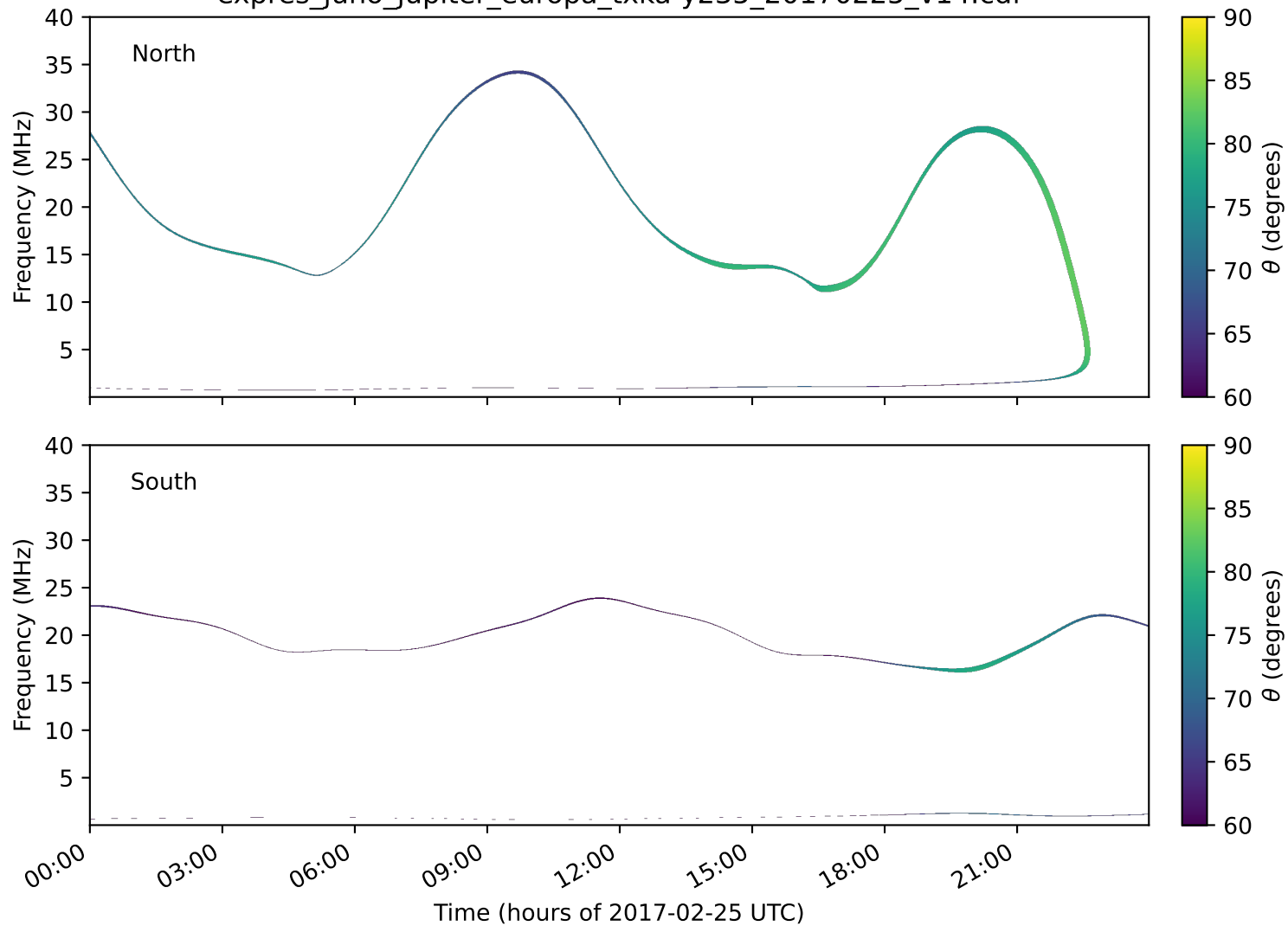
expres_juno_jupiter_europa_txka-y235_20170225_v14.cdf
