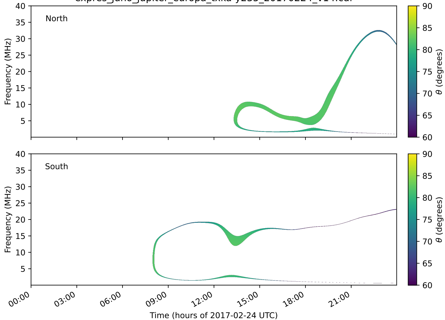
expres_juno_jupiter_europa_txka-y235_20170224_v14.cdf
