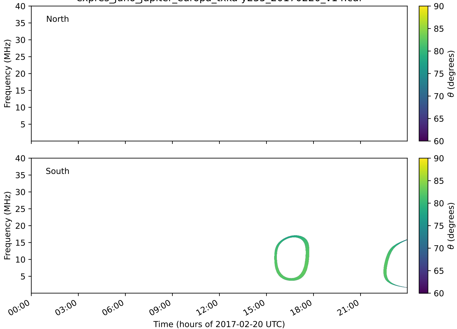
expres_juno_jupiter_europa_txka-y235_20170220_v14.cdf
