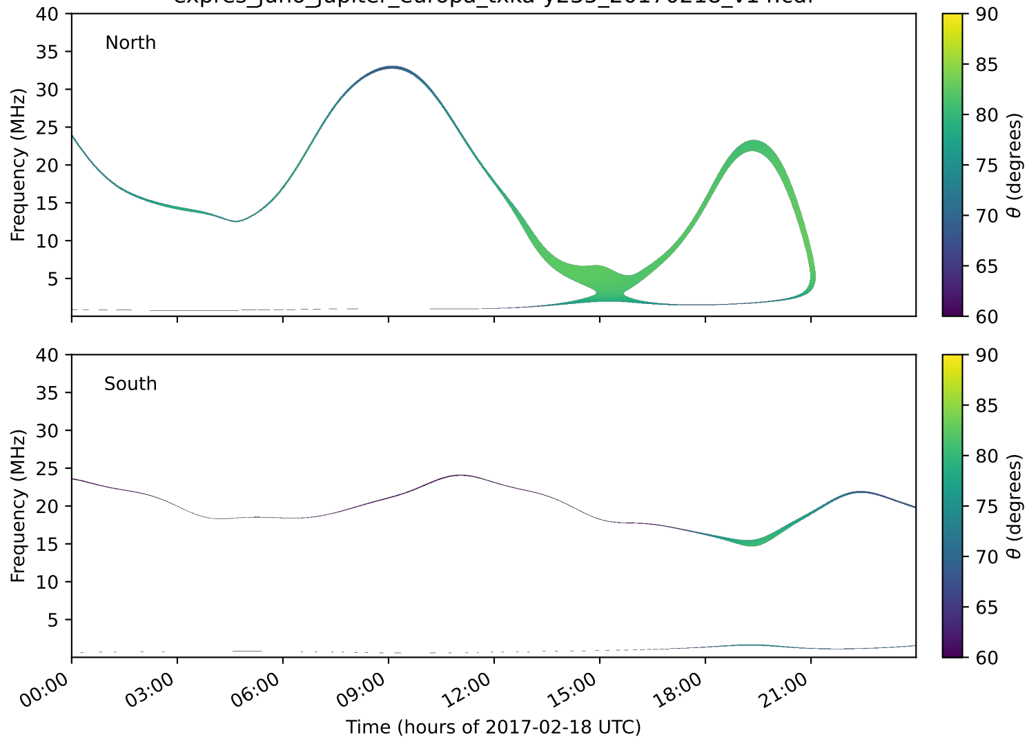
expres_juno_jupiter_europa_txka-y235_20170218_v14.cdf
