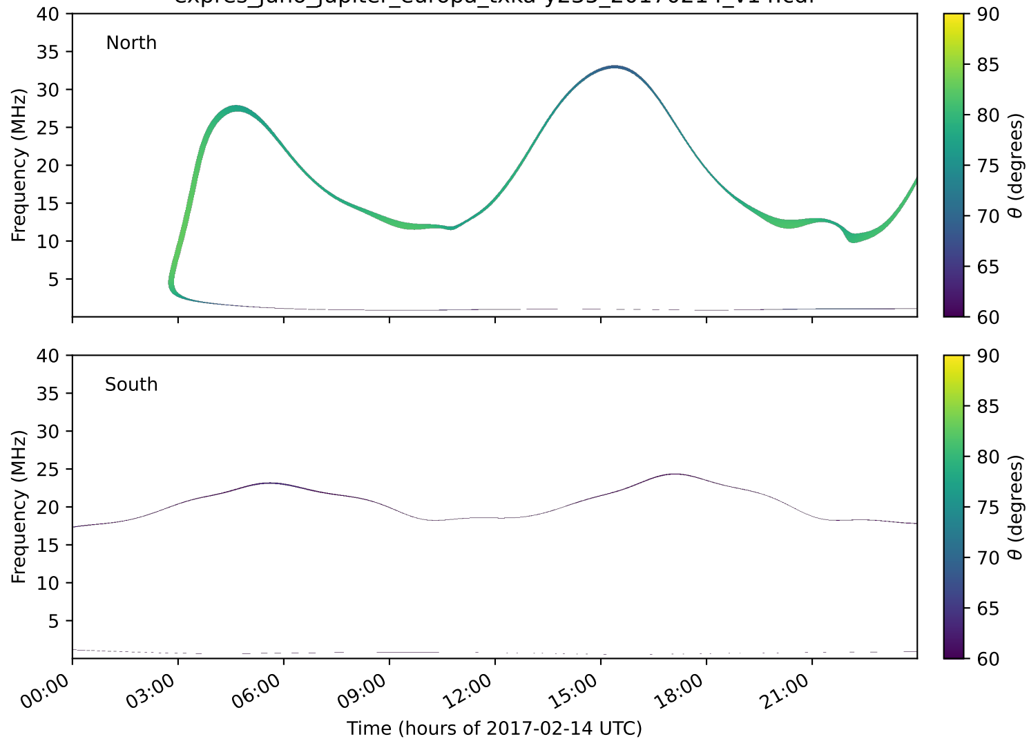
expres_juno_jupiter_europa_txka-y235_20170214_v14.cdf
