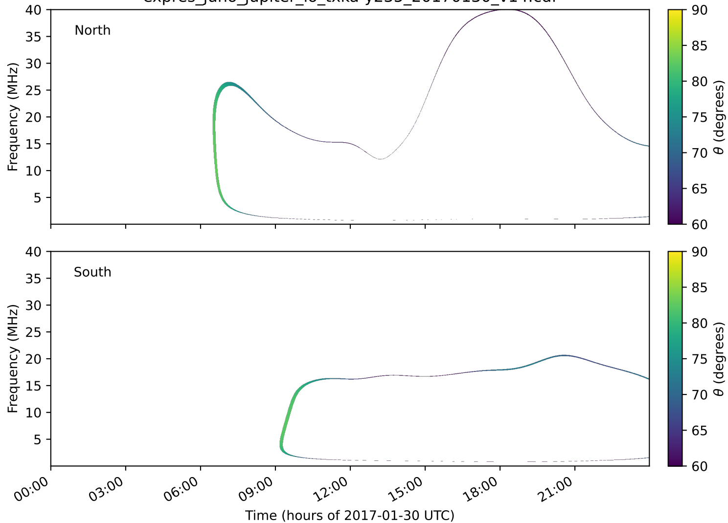
expres_juno_jupiter_io_txka-y235_20170130_v14.cdf
