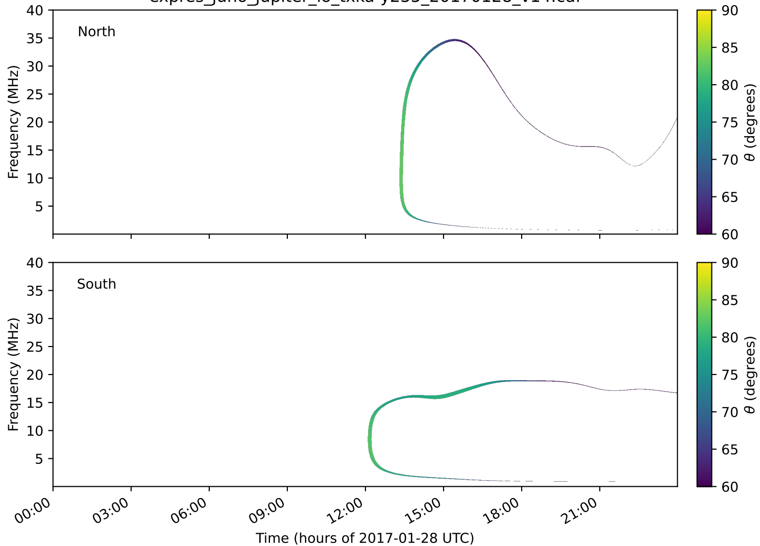
expres_juno_jupiter_io_txka-y235_20170128_v14.cdf
