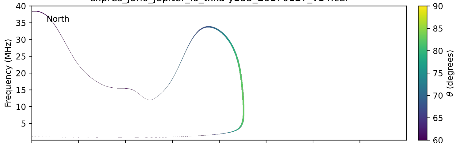
expres_juno_jupiter_io_txka-y235_20170127_v14.cdf
