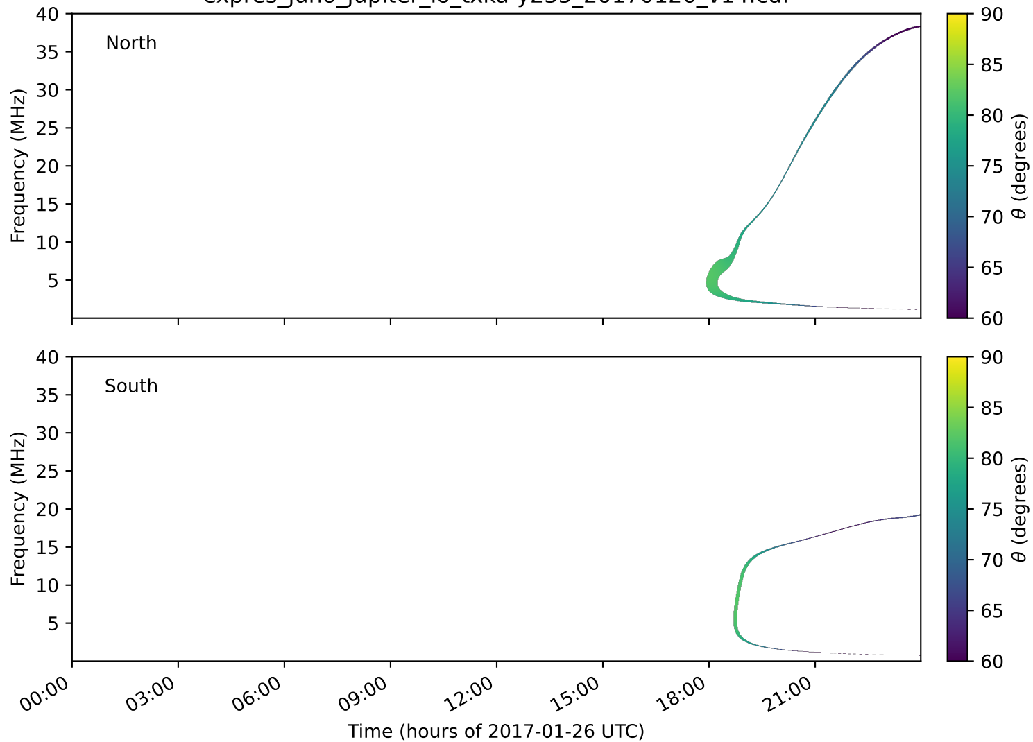
expres_juno_jupiter_io_txka-y235_20170126_v14.cdf
