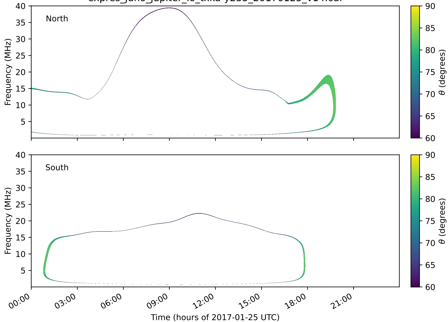
expres_juno_jupiter_io_txka-y235_20170125_v14.cdf
