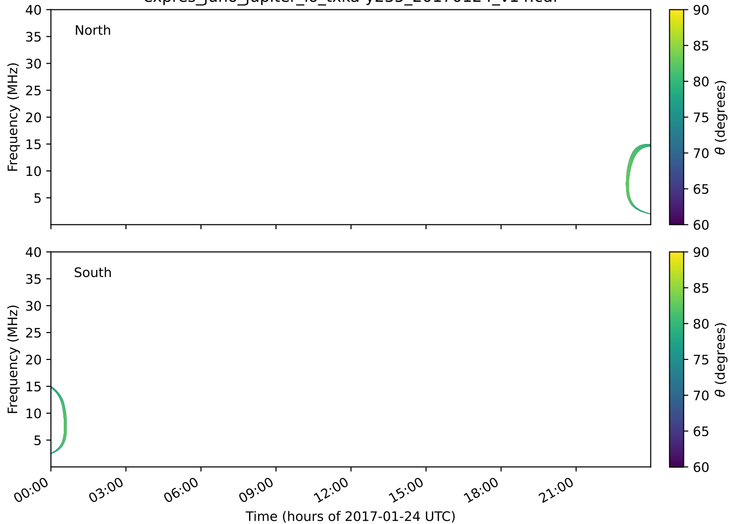
expres_juno_jupiter_io_txka-y235_20170124_v14.cdf
