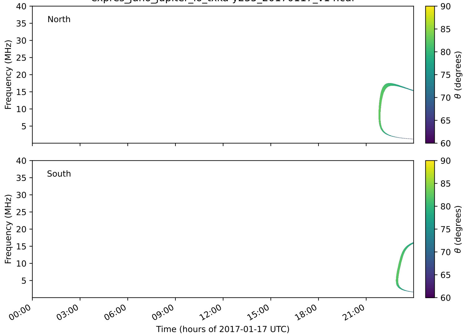
expres_juno_jupiter_io_txka-y235_20170117_v14.cdf
