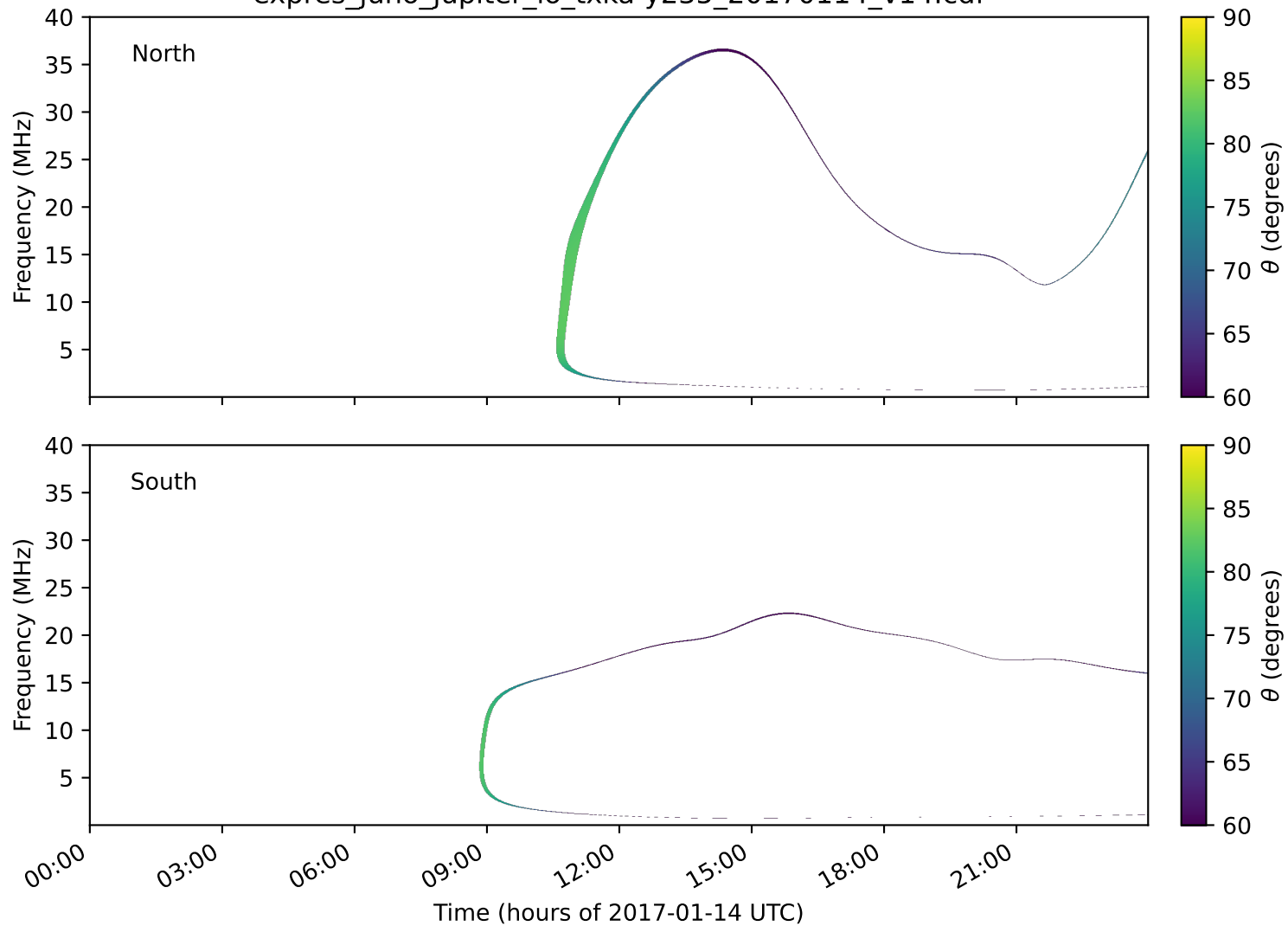
expres_juno_jupiter_io_txka-y235_20170114_v14.cdf
