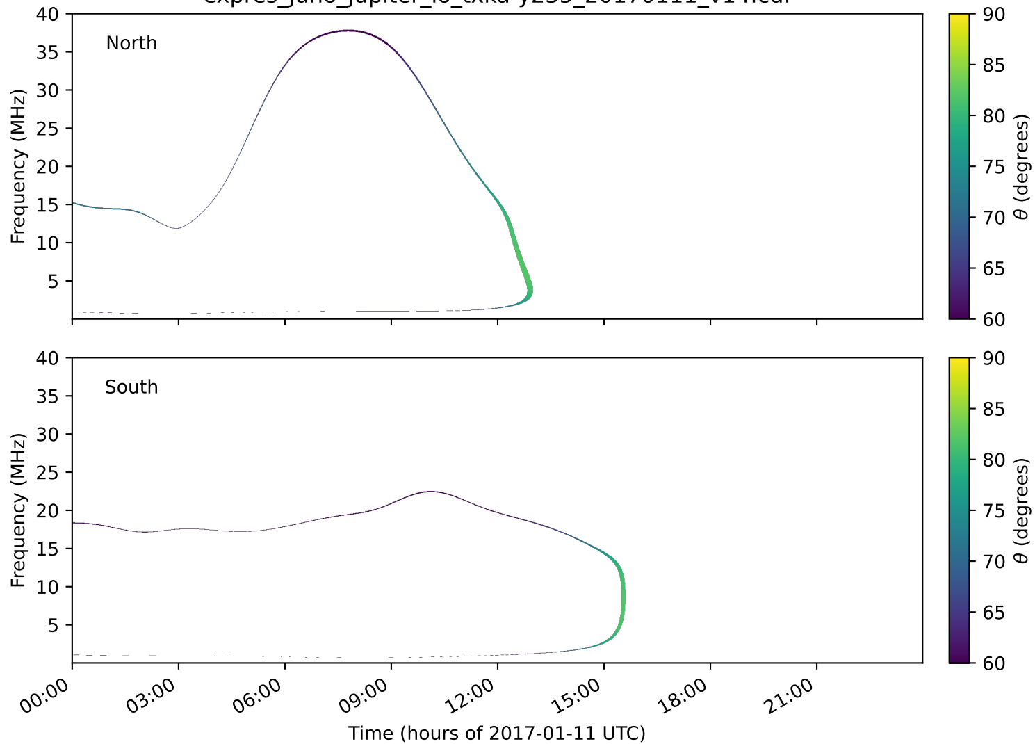
expres_juno_jupiter_io_txka-y235_20170111_v14.cdf
