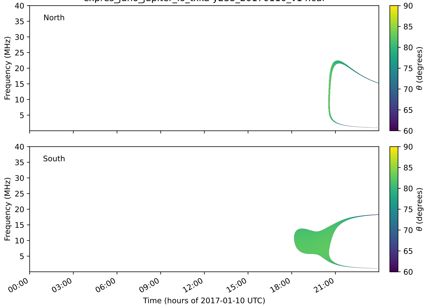
expres_juno_jupiter_io_txka-y235_20170110_v14.cdf
