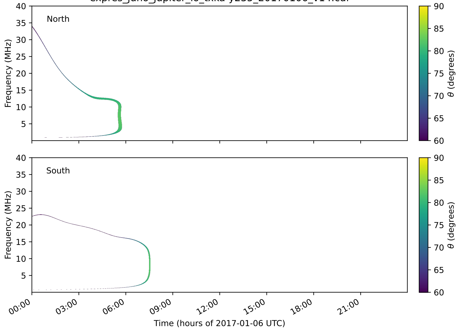
expres_juno_jupiter_io_txka-y235_20170106_v14.cdf
