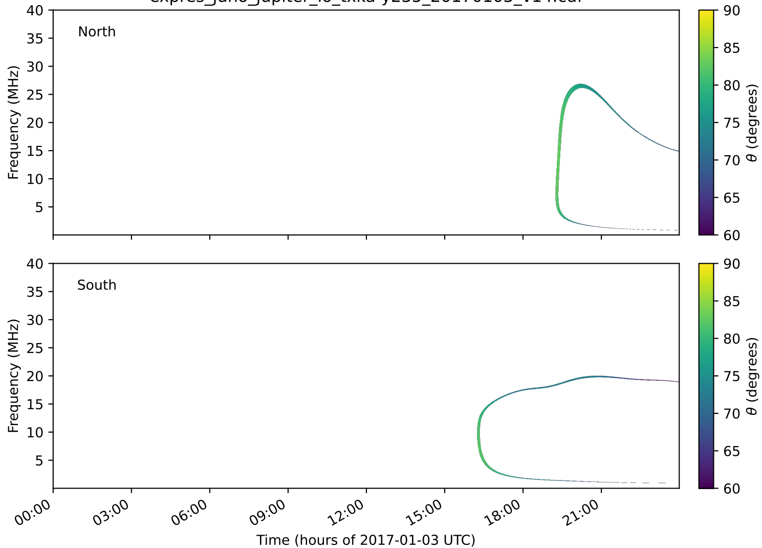
expres_juno_jupiter_io_txka-y235_20170103_v14.cdf
