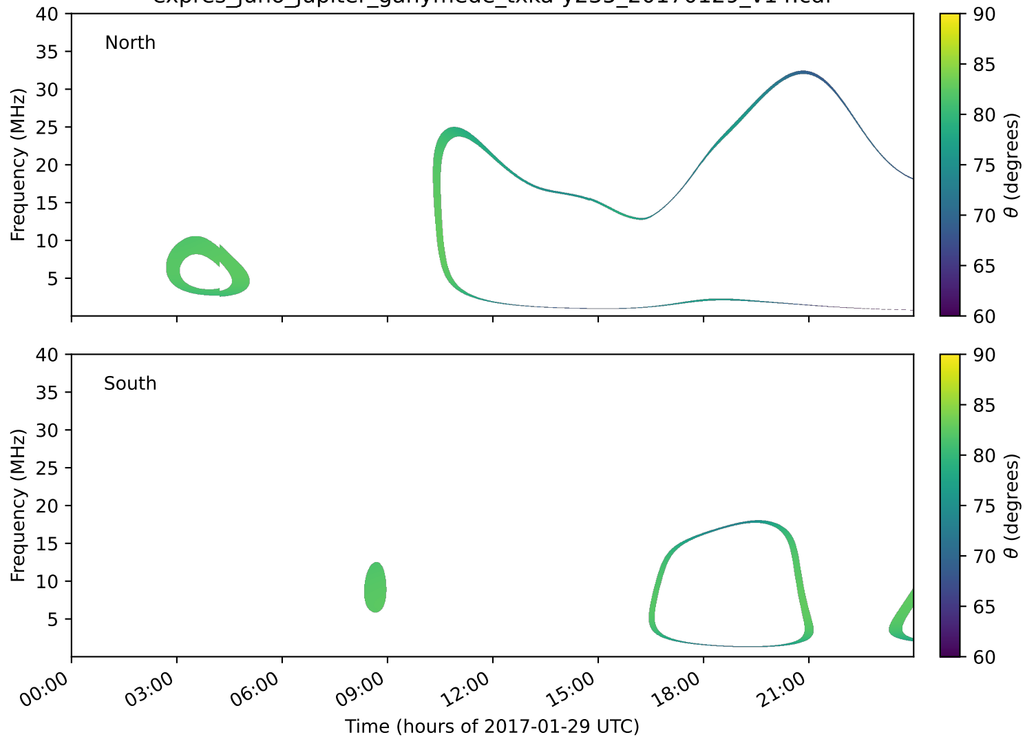
expres_juno_jupiter_ganymede_txka-y235_20170129_v14.cdf
