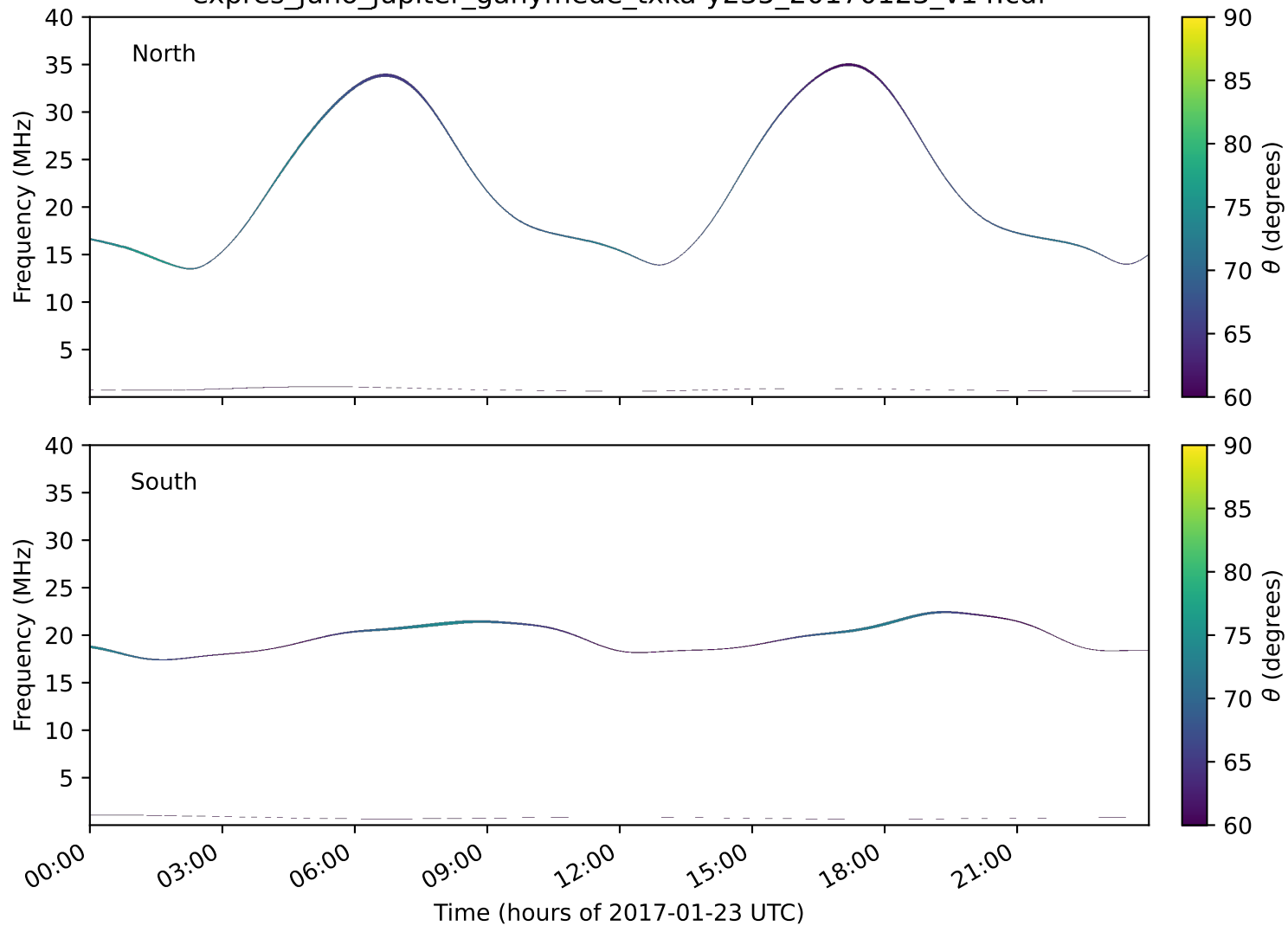
expres_juno_jupiter_ganymede_txka-y235_20170123_v14.cdf
