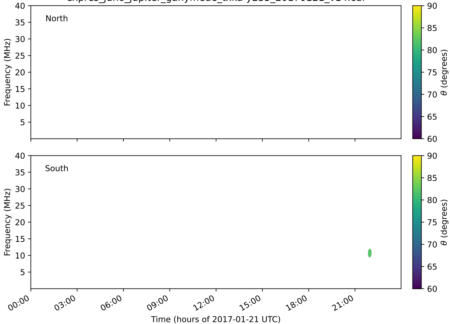
expres_juno_jupiter_ganymede_txka-y235_20170121_v14.cdf
