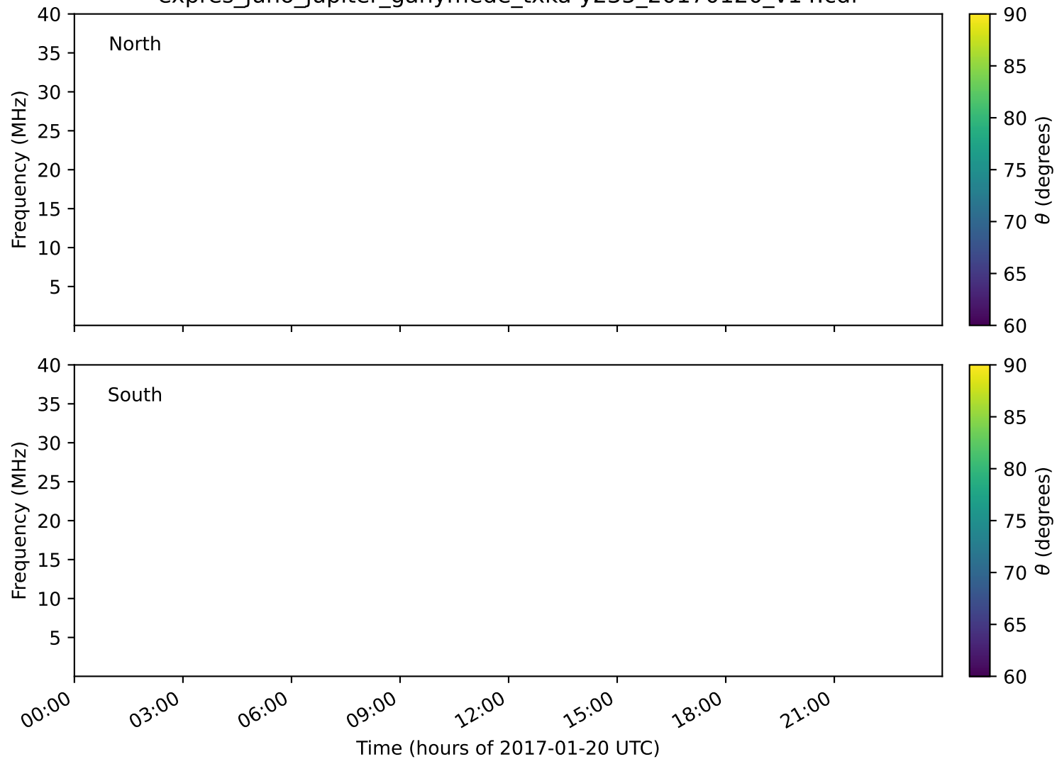
expres_juno_jupiter_ganymede_txka-y235_20170120_v14.cdf
