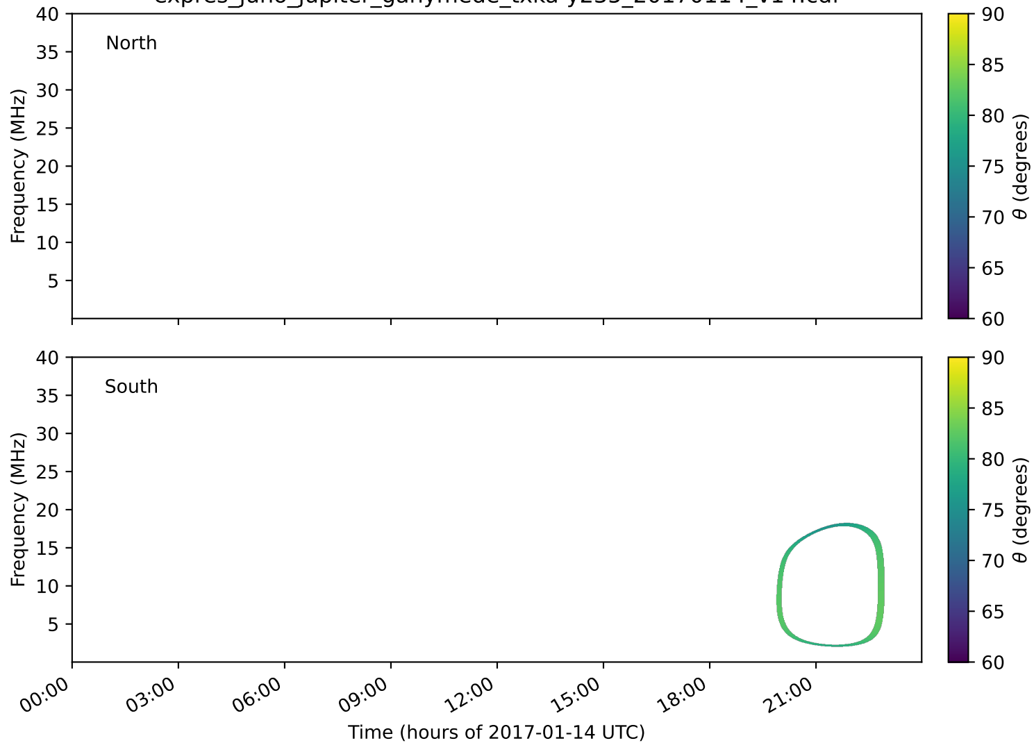
expres_juno_jupiter_ganymede_txka-y235_20170114_v14.cdf
