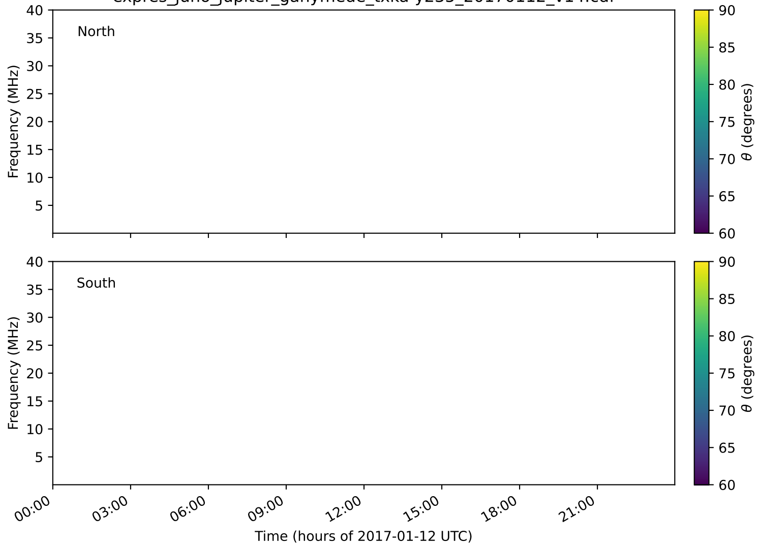
expres_juno_jupiter_ganymede_txka-y235_20170112_v14.cdf
