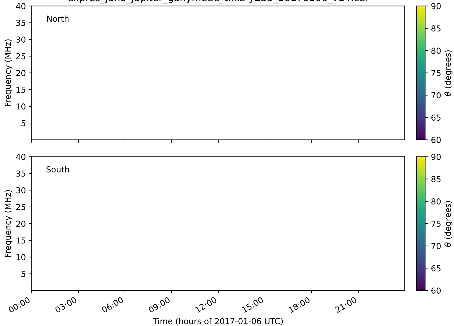
expres_juno_jupiter_ganymede_txka-y235_20170106_v14.cdf
