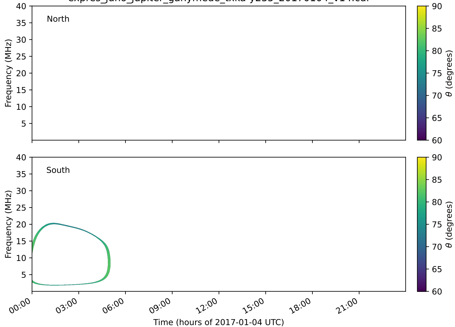
expres_juno_jupiter_ganymede_txka-y235_20170104_v14.cdf
