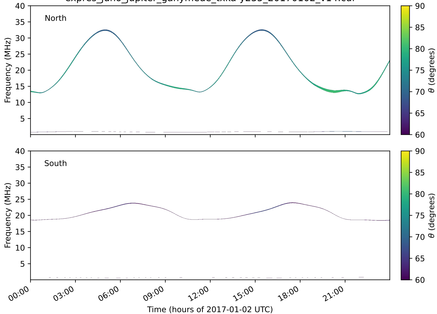
expres_juno_jupiter_ganymede_txka-y235_20170102_v14.cdf
