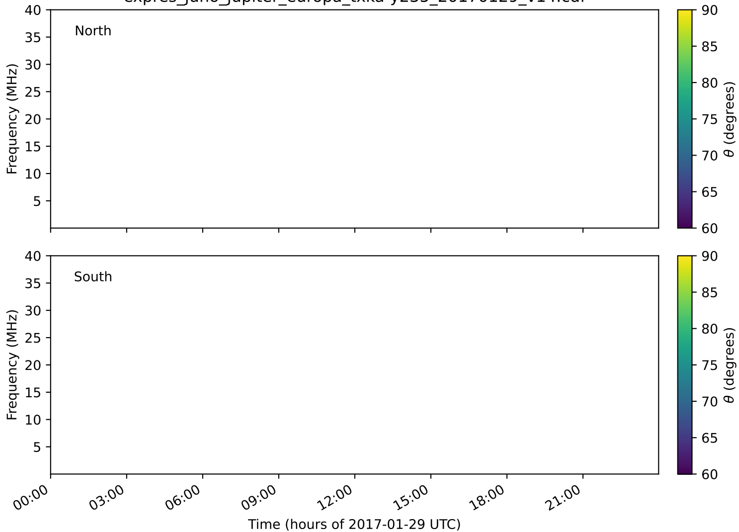
expres_juno_jupiter_europa_txka-y235_20170129_v14.cdf
