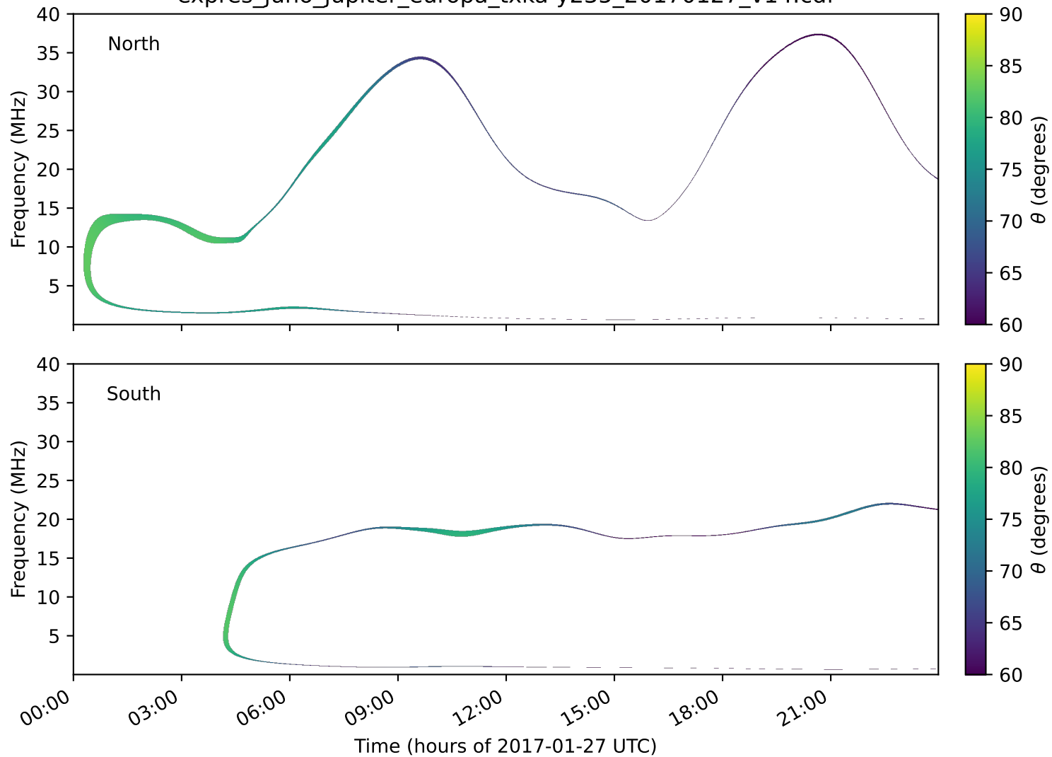
expres_juno_jupiter_europa_txka-y235_20170127_v14.cdf
