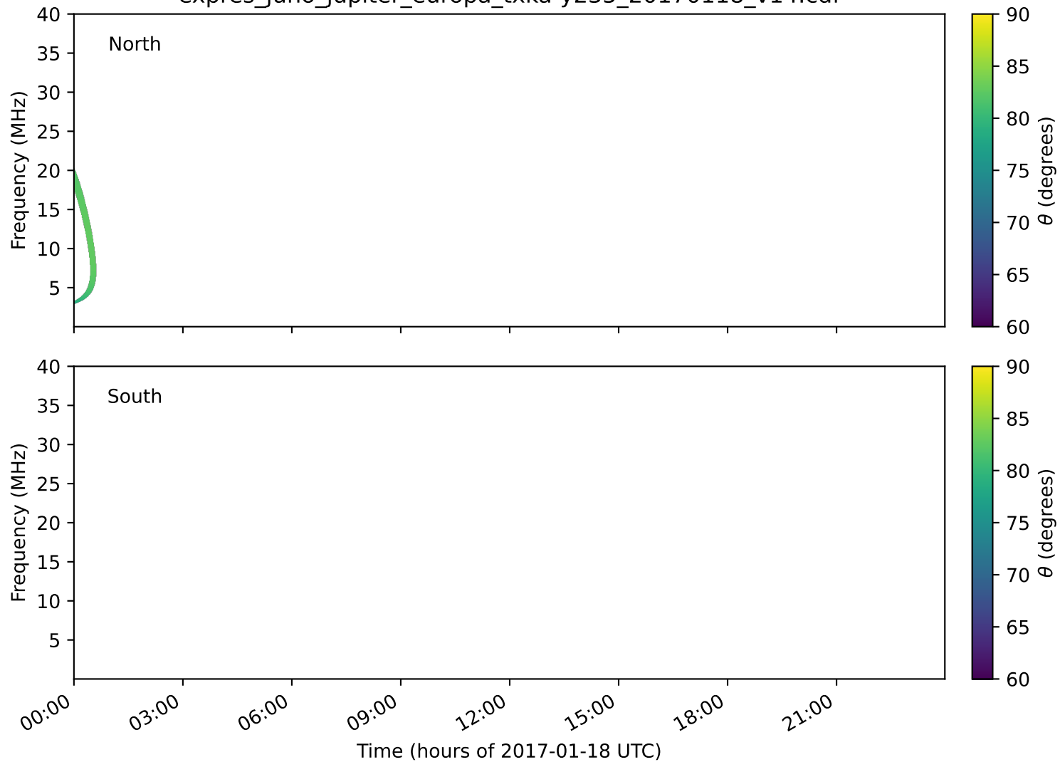
expres_juno_jupiter_europa_txka-y235_20170118_v14.cdf
