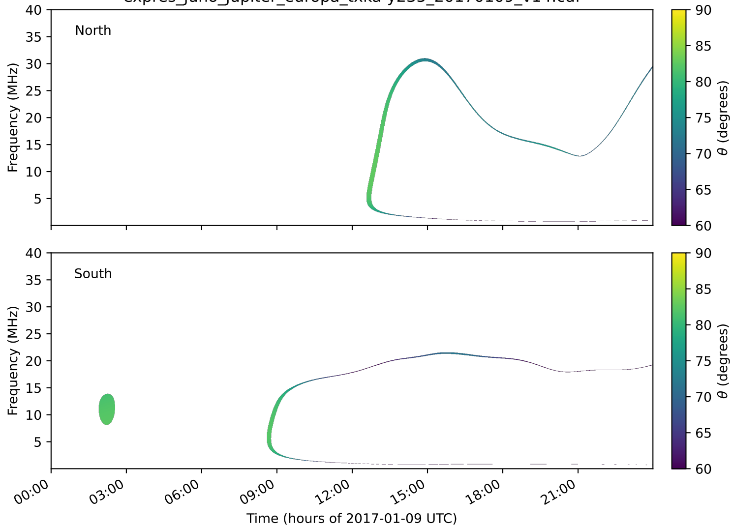
expres_juno_jupiter_europa_txka-y235_20170109_v14.cdf
