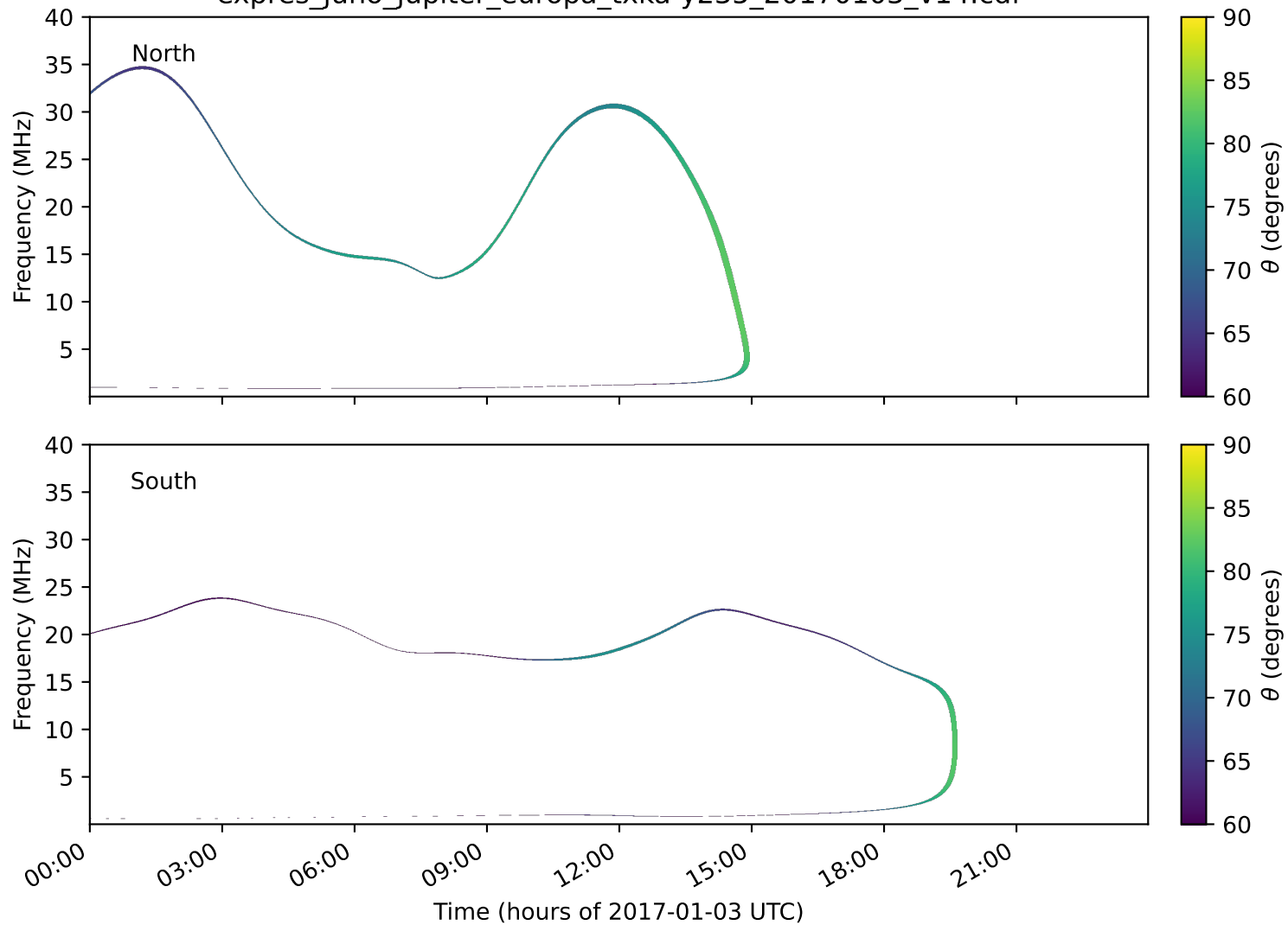
expres_juno_jupiter_europa_txka-y235_20170103_v14.cdf
