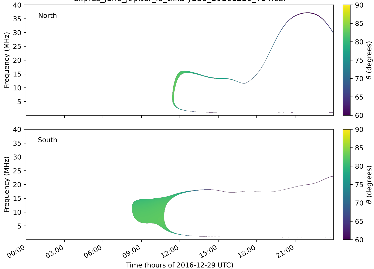
expres_juno_jupiter_io_txka-y235_20161229_v14.cdf
