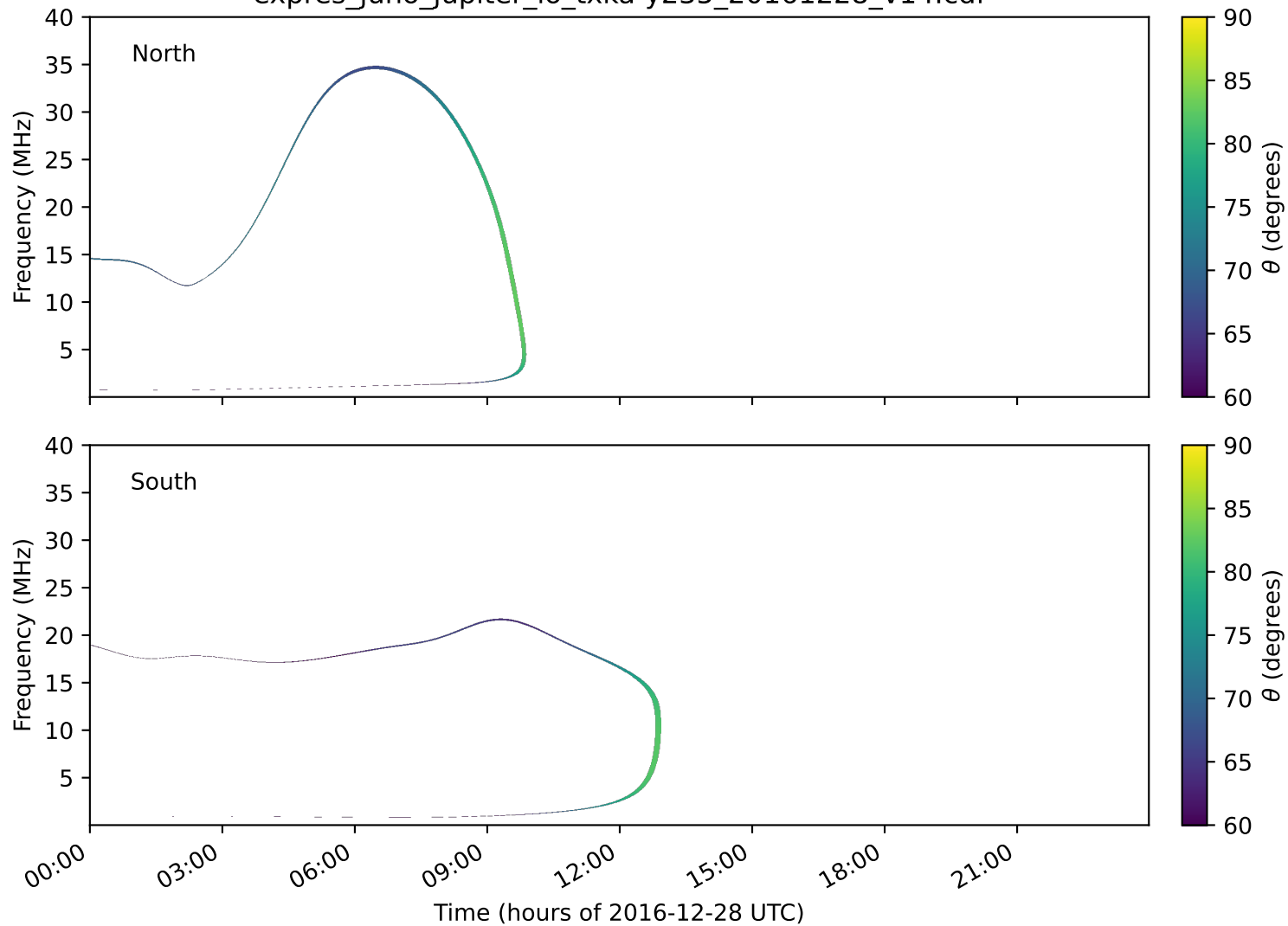
expres_juno_jupiter_io_txka-y235_20161228_v14.cdf
