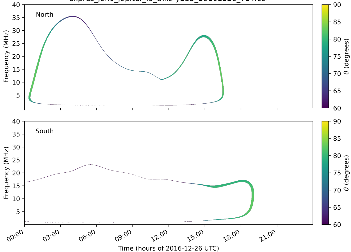
expres_juno_jupiter_io_txka-y235_20161226_v14.cdf
