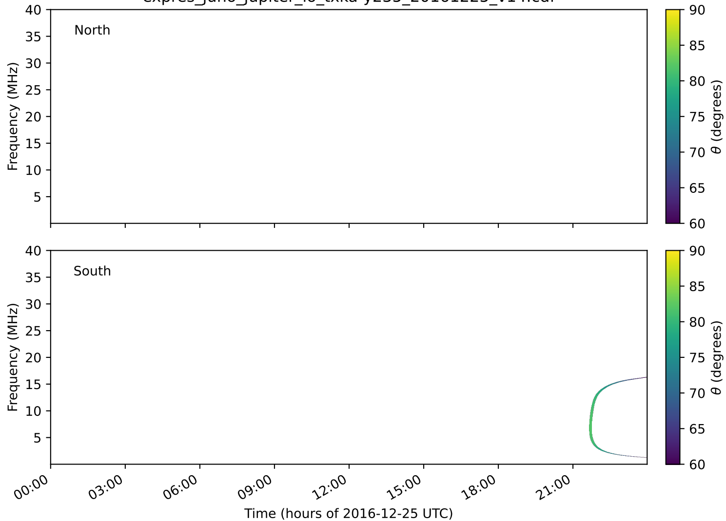
expres_juno_jupiter_io_txka-y235_20161225_v14.cdf
