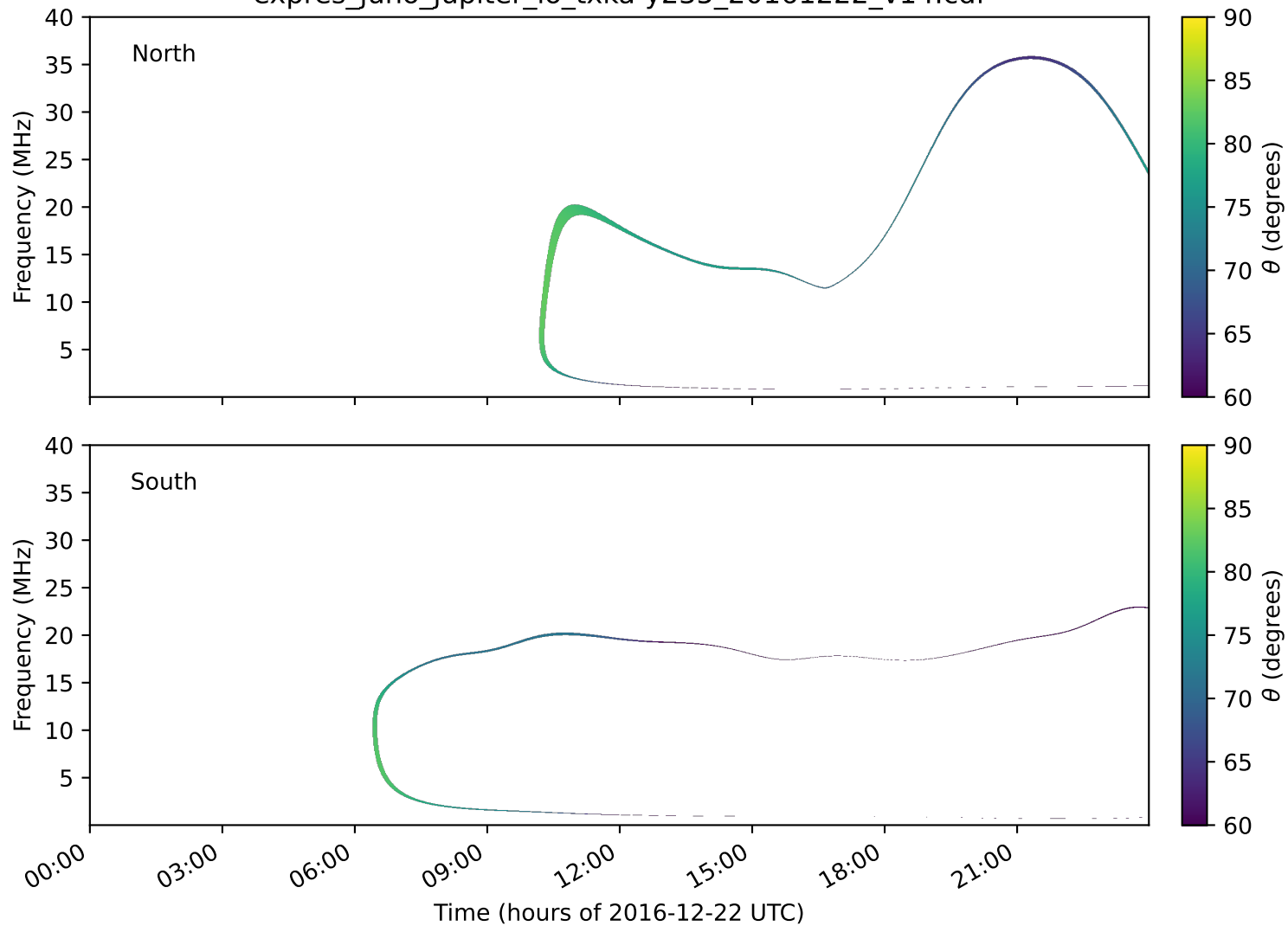
expres_juno_jupiter_io_txka-y235_20161222_v14.cdf
