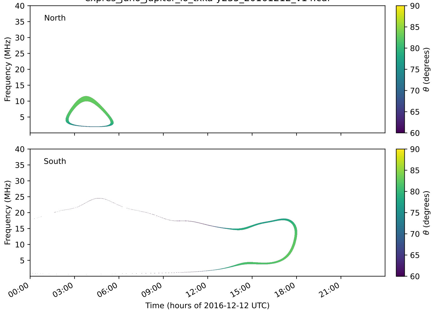
expres_juno_jupiter_io_txka-y235_20161212_v14.cdf
