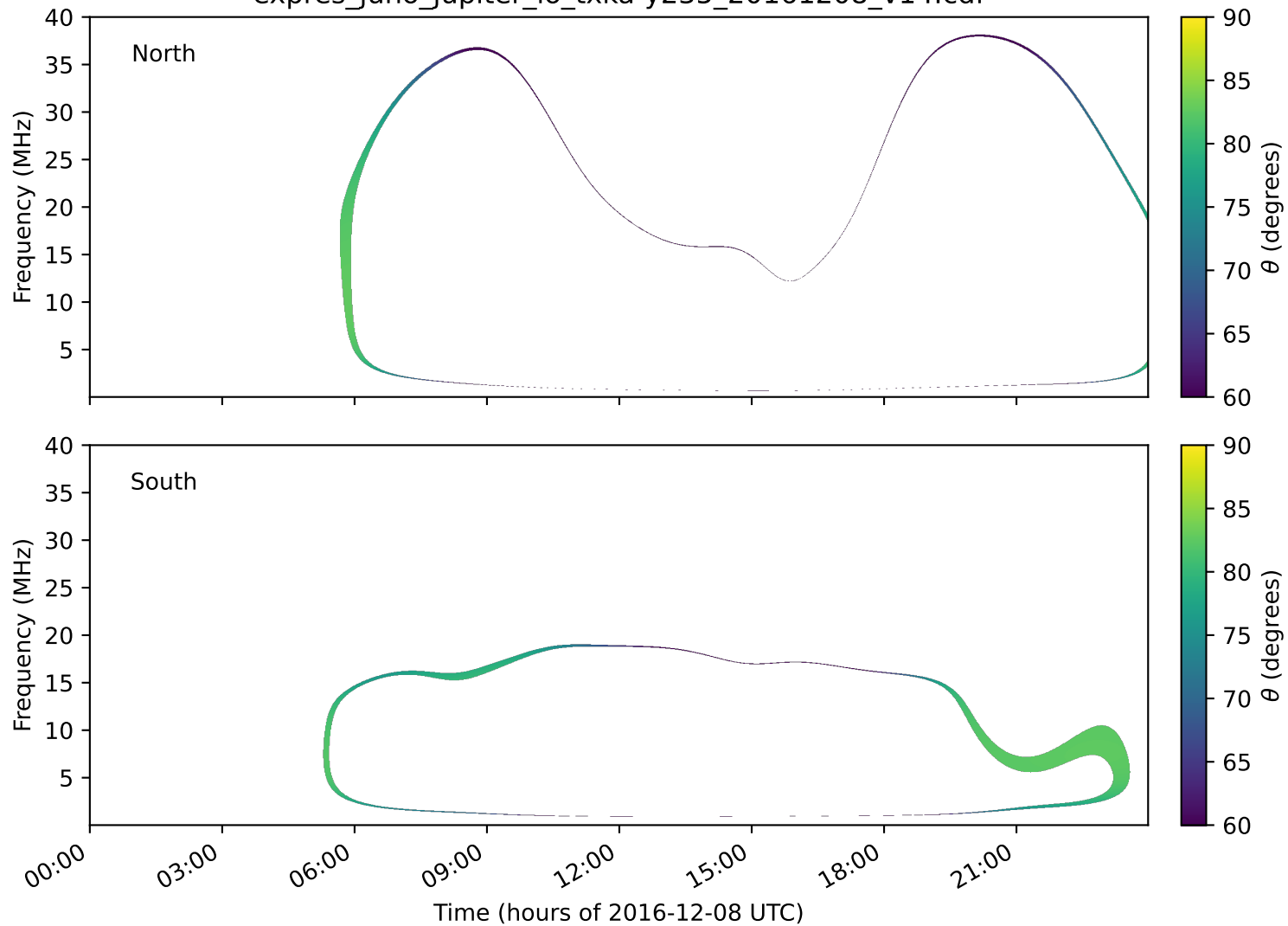
expres_juno_jupiter_io_txka-y235_20161208_v14.cdf
