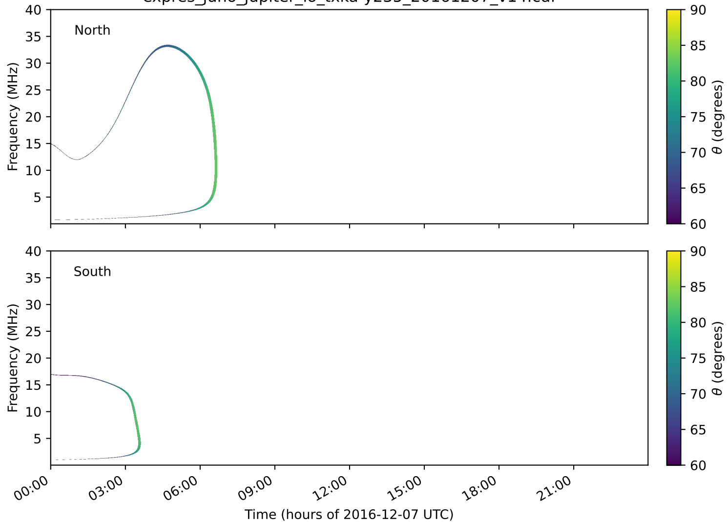
expres_juno_jupiter_io_txka-y235_20161207_v14.cdf
