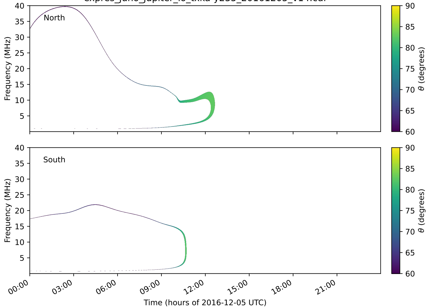
expres_juno_jupiter_io_txka-y235_20161205_v14.cdf
