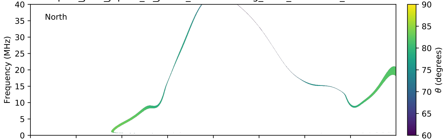
expres_juno_jupiter_io_jrm09_lossc-wid1deg_3kev_20161231_v01.cdf
