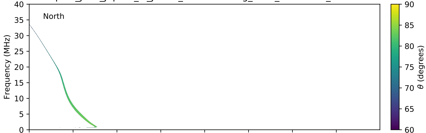
expres_juno_jupiter_io_jrm09_lossc-wid1deg_3kev_20161230_v01.cdf
