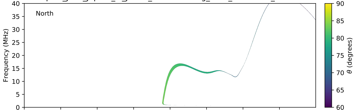
expres_juno_jupiter_io_jrm09_lossc-wid1deg_3kev_20161229_v01.cdf
