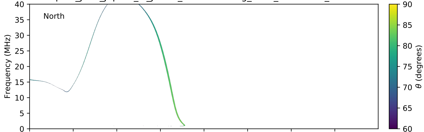
expres_juno_jupiter_io_jrm09_lossc-wid1deg_3kev_20161228_v01.cdf
