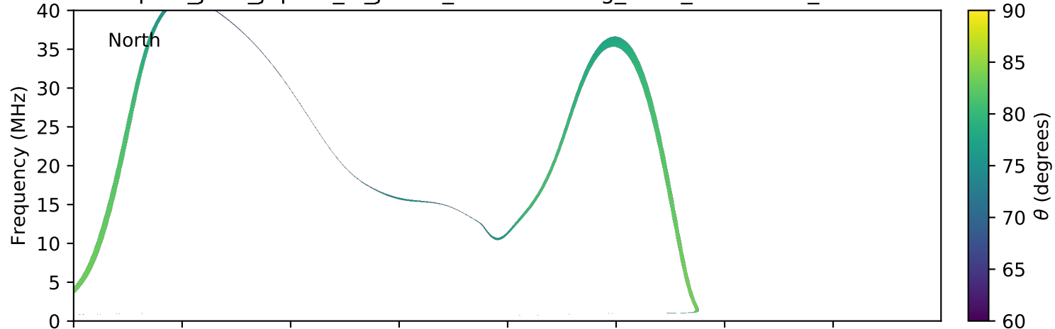
expres_juno_jupiter_io_jrm09_lossc-wid1deg_3kev_20161226_v01.cdf
