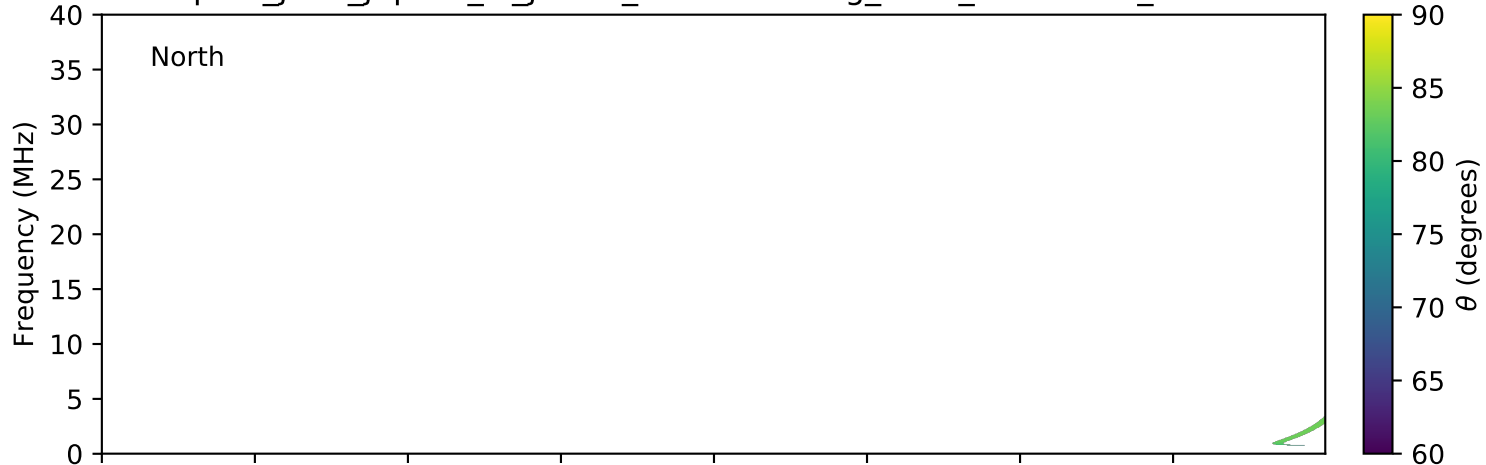
expres_juno_jupiter_io_jrm09_lossc-wid1deg_3kev_20161225_v01.cdf
